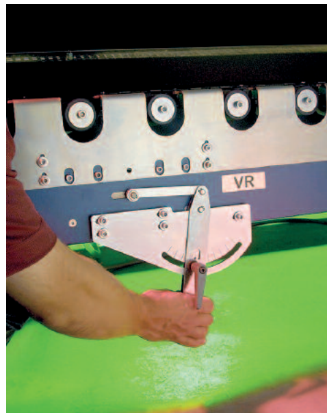
Quick adjustment for frame setback
